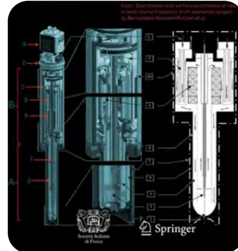
HIGH-POWER SPALLATION TARGET (6+ MO OPERATION)
